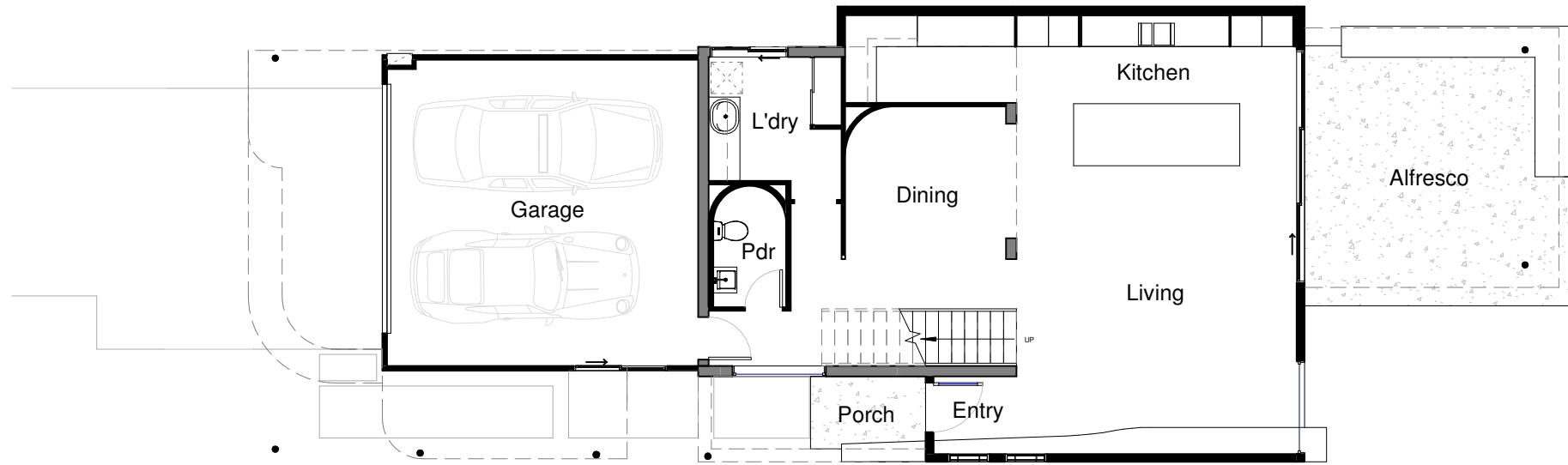
1 Ground Floor 1 : 100
